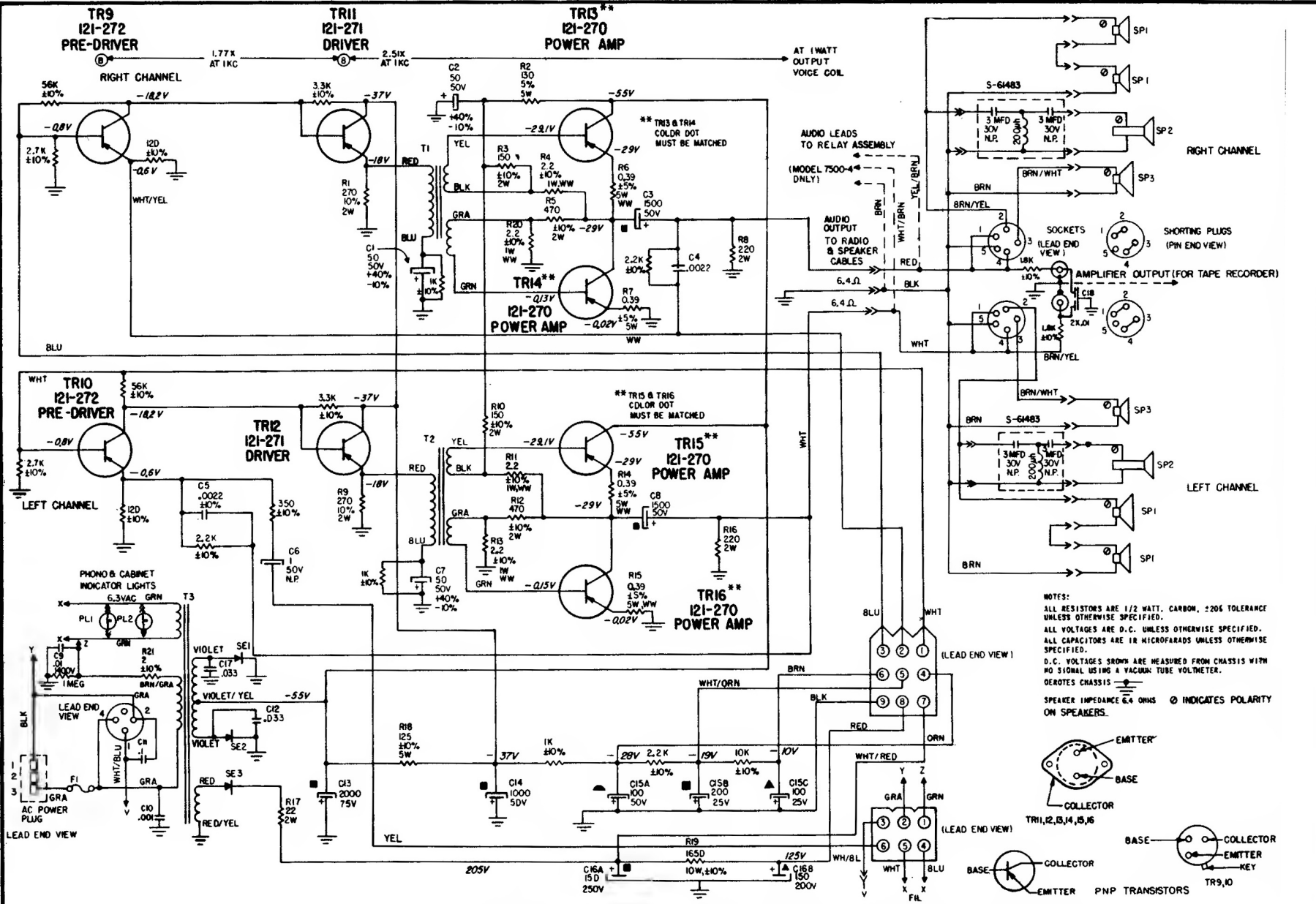
ZENITH 8L25Z SCHEMATIC FOR MODELS ML2670-3, ML2675-3, ML2685-3 AND 7500-3
